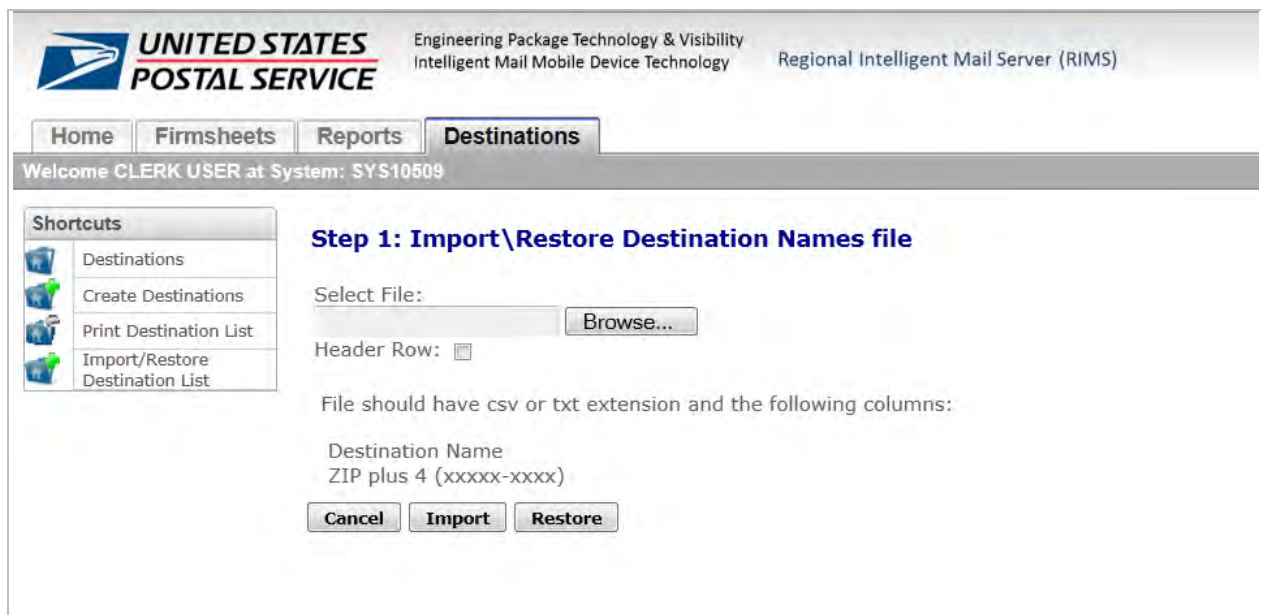
Figure 21. Destinations Tab - Import/Restore Destinations List
