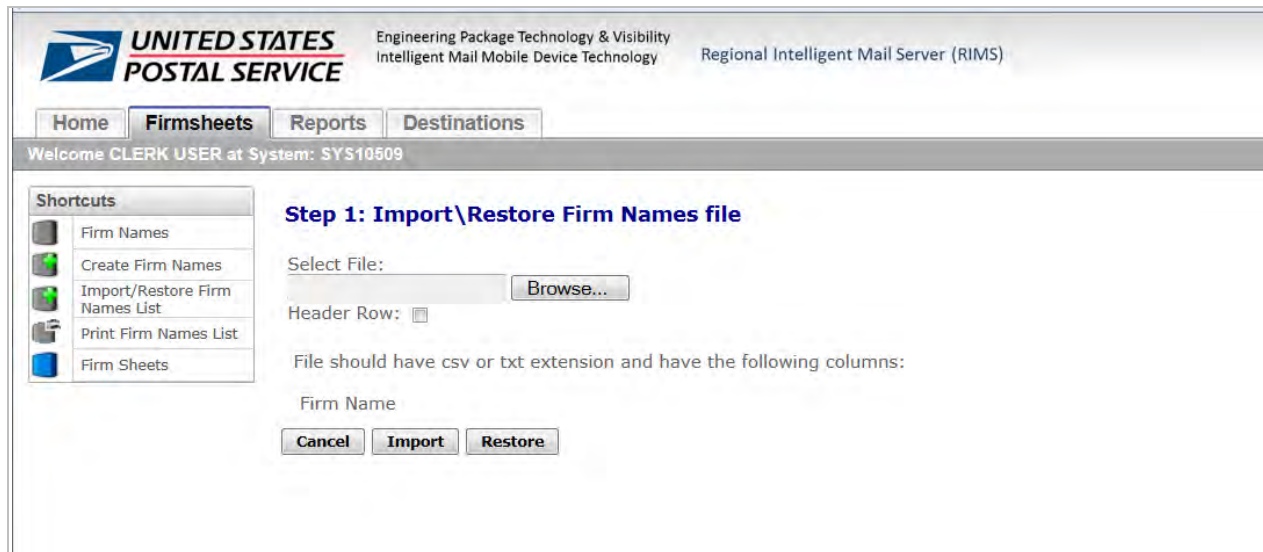
Figure 9. Firmsheets Tab - Import/Restore Firm Names File
